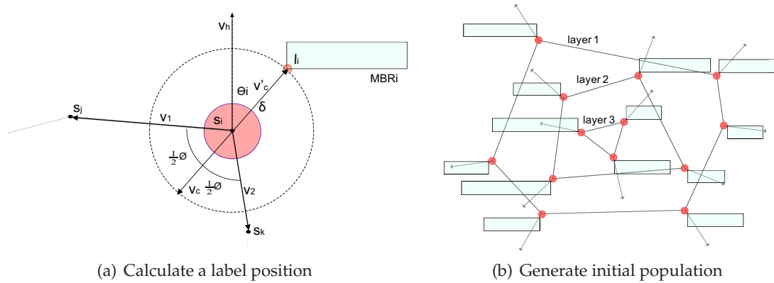
Figure 5: Label positions using convex onion peeling
