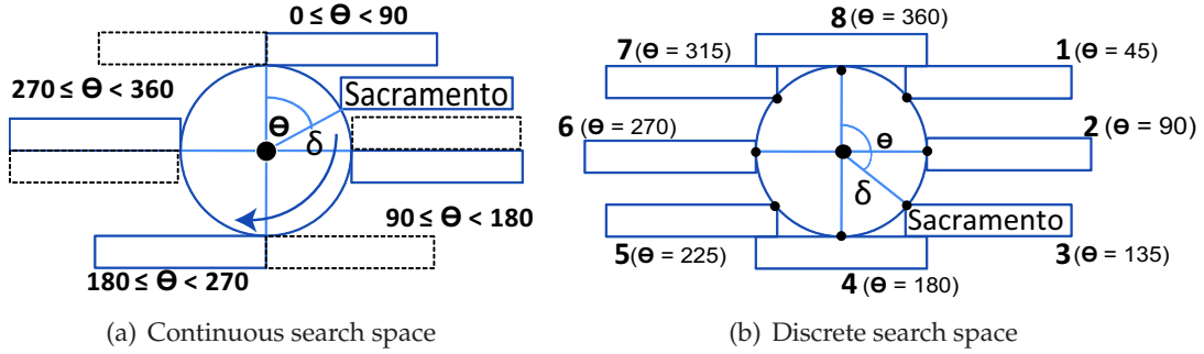
Figure 3: Search space for label positions
