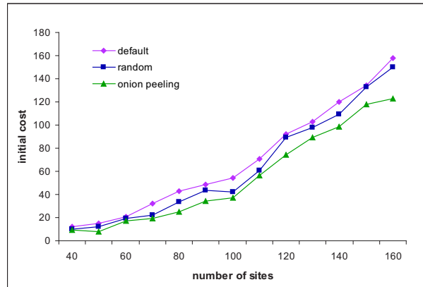
Figure 9: Map initialization
