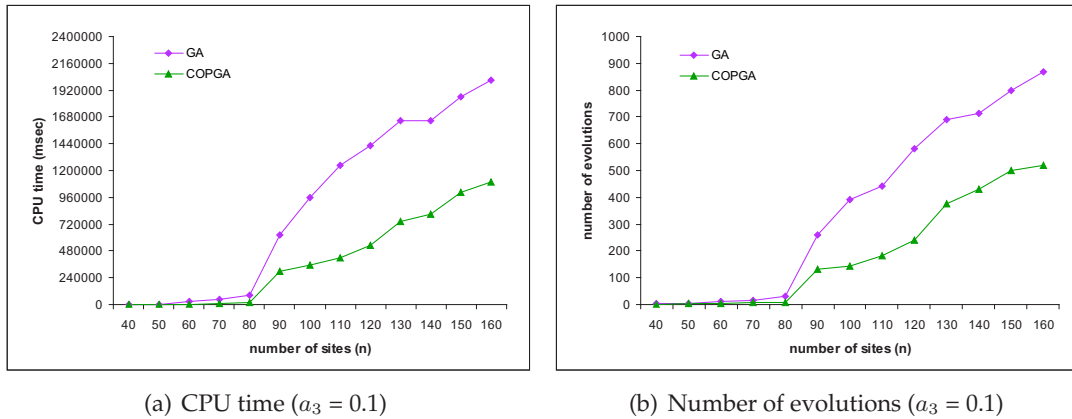
Figure 12: Comparison of COPGA and GA w/synthetic datasets
