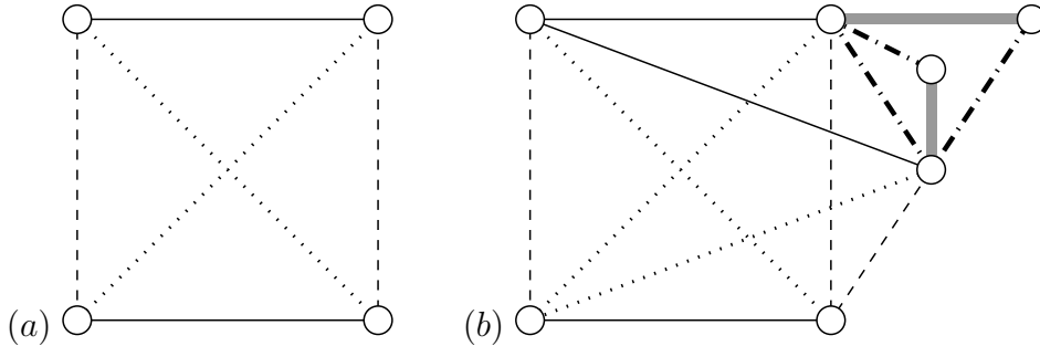
FIGURE 1. Restricted graphs giving lower bounds for Proposition 8.1.
