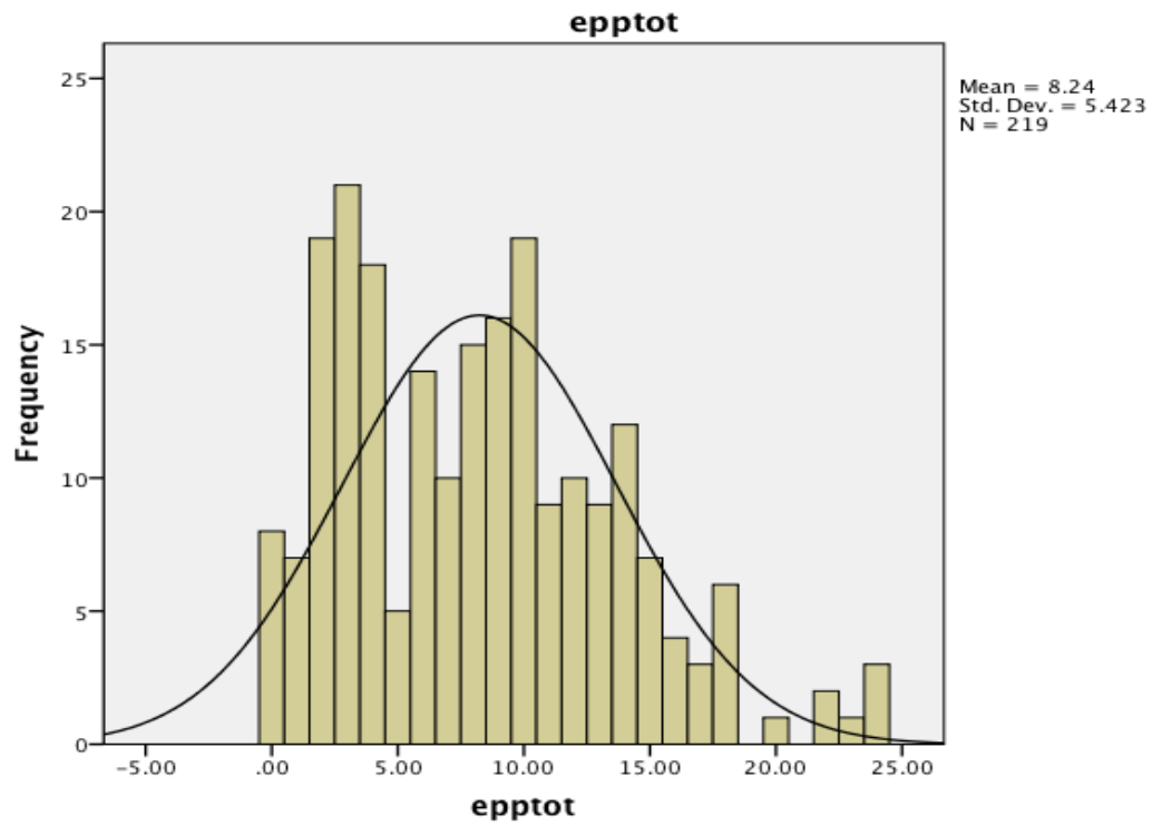
Figure 3. Distribution of the Epworth Sleepiness Scale
