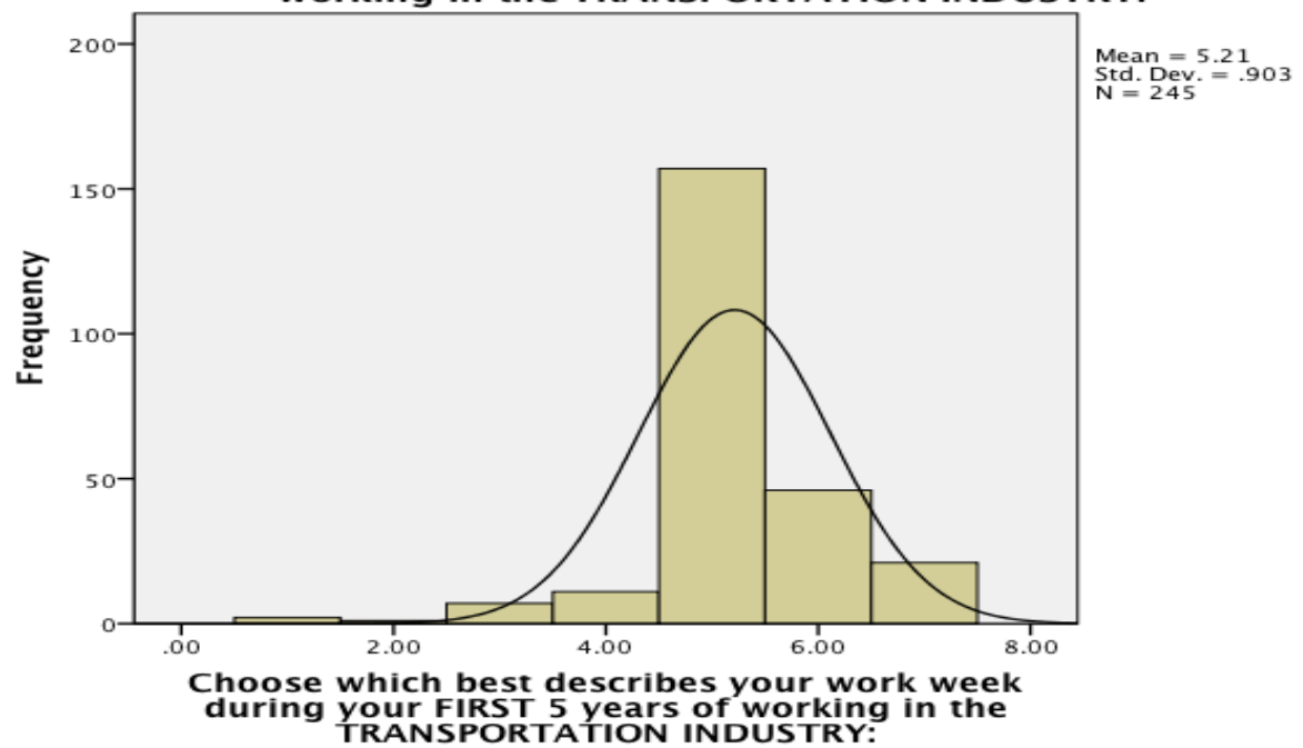
Figure 10. Frequency distribution for Total Days Worked During First 5 Years
