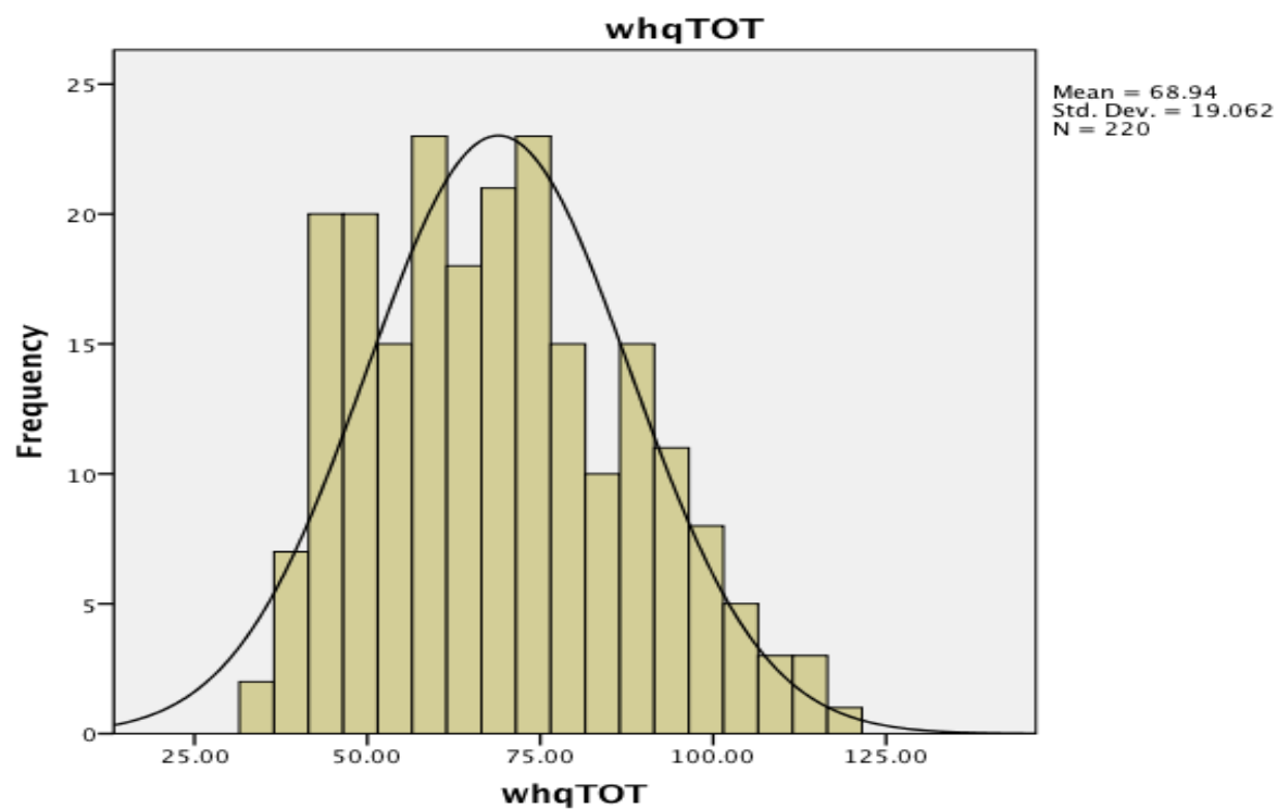
Figure 5. Distribution of the Women's Health Questionnaire.
