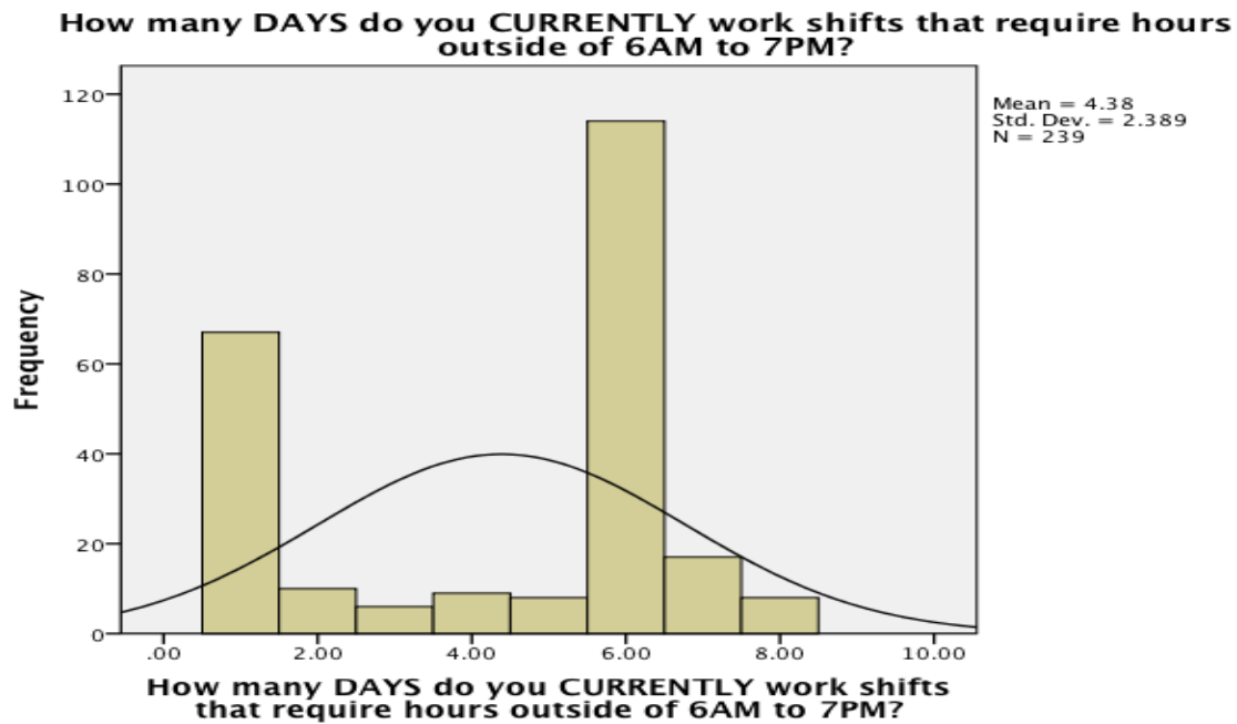
Figure 14. Frequency of Total Current Days of Working Shift Work
