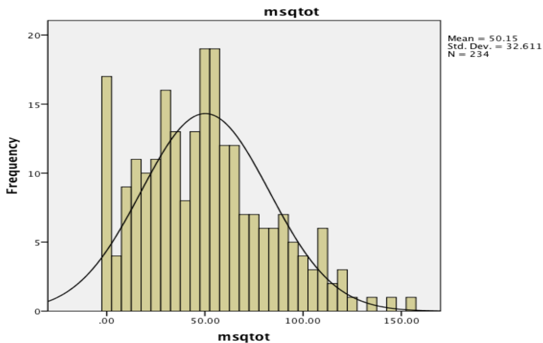
Figure 4. Distribution of the Menstrual Distress Questionnaire
